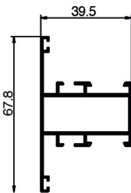
▶ 516 Weight: 0.680 KG/M
