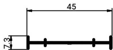
▶ 3637 Weight: 0.213 KG/M
