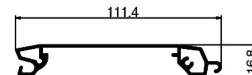
▶ 1202 Weight: 0.730 KG/M
