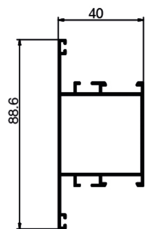
▶ 517 Weight: 0.780 KG/M
