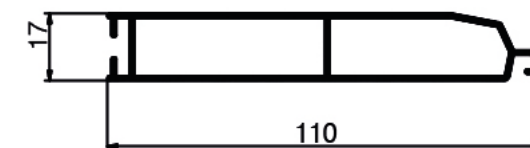
▶ 1201 Weight: 0.875 KG/M
