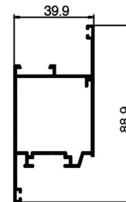
▶ 1.070 Weight: 0.785 KG/M
