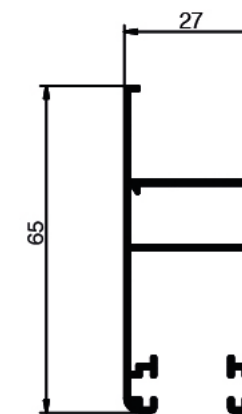
▶ 1.157 Weight: 0.665 KG/M
