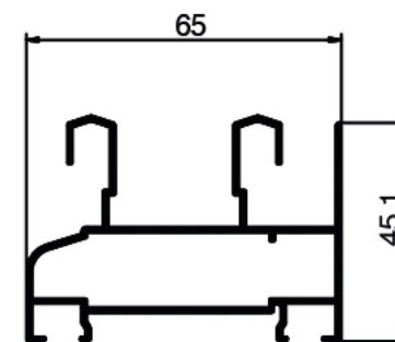
▶ 1.156 Weight: 0.883 KG/M
