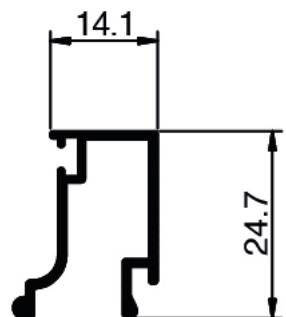
▶ 502 Weight: 0.229 KG/M
