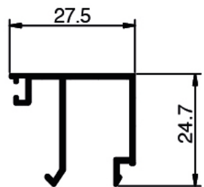
▶ 501 Weight: 0.265 KG/M
