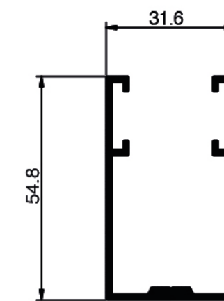
▶ 1200 Weight: 0.702 KG/M
