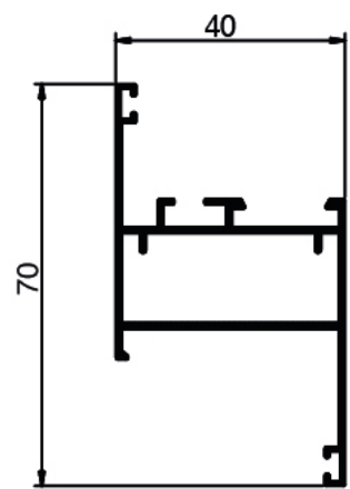
▶ 548 Weight: 0.625 KG/M
