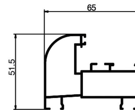
▶ 1.161 Weight: 0.840 KG/M
