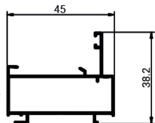
▶ 3937 Weight: 0.440 KG/M
