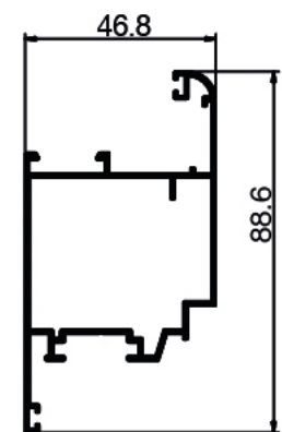
▶ 514 Weight: 0.855 KG/M
