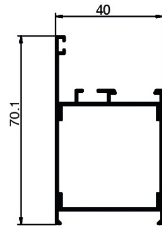
▶ 903 Weight: 0.735 KG/M
