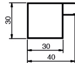
IF 132 Weight: 0.261 KG/M
