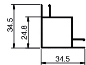
IF 131 Weight: 0.260 KG/M
