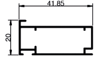
IF 566 Weight: 0.260 KG/M
