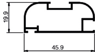
IF 552 Weight: 0.278 KG/M
