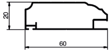
IF 522 Weight: 0.337 KG/M
