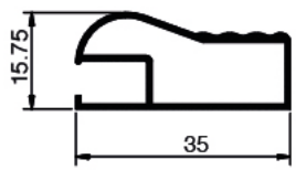
IF 550 A Weight: 0.228 KG/M
