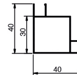
IF 138 Weight: 0.302 KG/M
