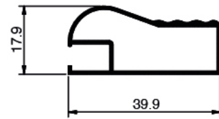
IF 550 Weight: 0.248 KG/M
