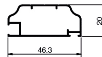
IF 587 Weight: 0.264 KG/M
