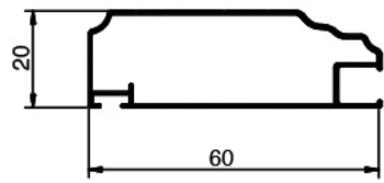
IF 523 Weight: 0.337 KG/M
