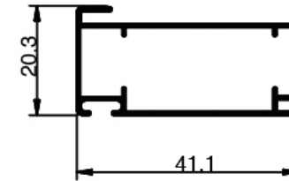
IF 567 Weight: 0.275 KG/M
