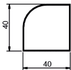
IF 120 Weight: 0.264 KG/M
