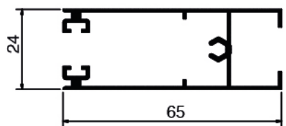
NC 1216 Weight: 0.494 KG/M
