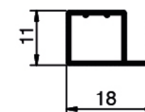
NC 1517 Weight: 0.125 KG/M
