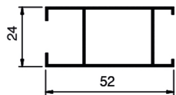
NC 1221 Weight: 0.313 KG/M
