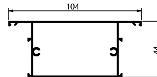
NC 1376 B Weight: 0.730 KG/M
