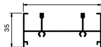
NC 1227 Weight: 0.650 KG/M
