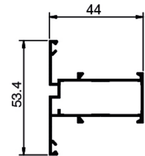
NC 1373 Weight: 0.425 KG/M
