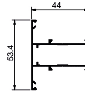
NC 1372 Weight: 0.425 KG/M
