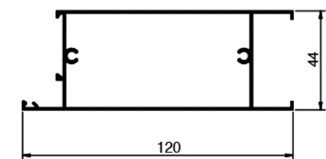
NC 1380 Weight: 0.950 KG/M
