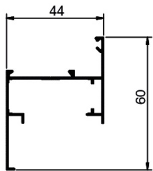
NC 1369 Weight: 0.335 KG/M
