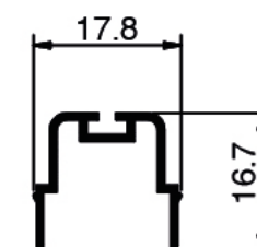
NC 1503 Weight: 0.108 KG/M
