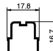
NC 1504 Weight: 0.100 KG/M
