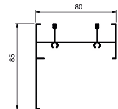
NC 1340A Weight: 0.728 KG/M
