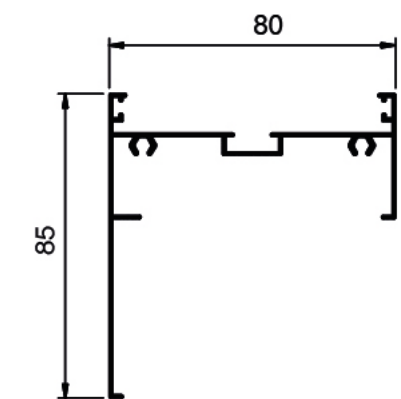
NC 1339A Weight: 0.595 KG/M
