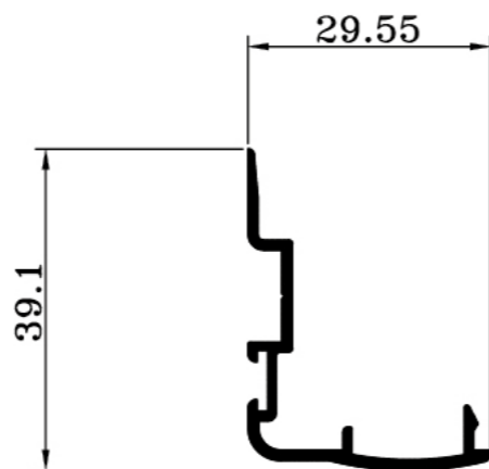
▶ JS 6050 Weight: 0.285 KG/M
