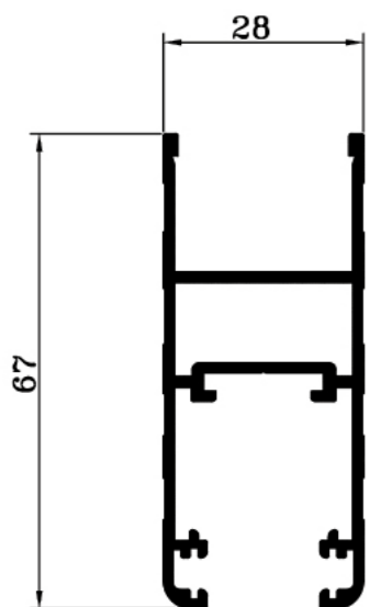
▶ JS 6042 Weight: 0.850 KG/M
