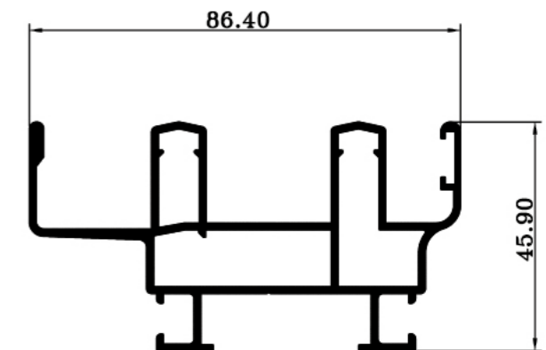
▶ JS 6023 Weight: 1.370 KG/M
