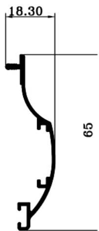
▶ JS 6085 Weight: 0.347 KG/M
