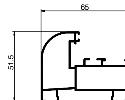
1.161 Weight: 0.840 KG/M
