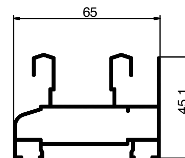
1.156 Weight: 0.883 KG/M
