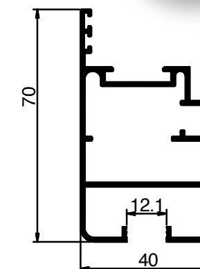
▶ HSB 17 Weight: 0.904 KG/M
