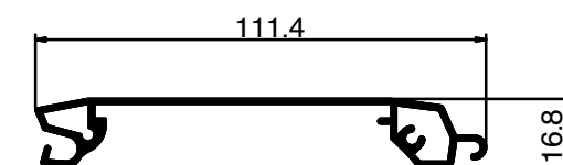
1202 Weight: 0.730 KG/M
