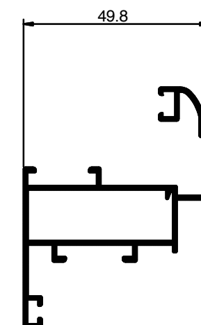
MR 705 Weight: 0.750 KG/M
