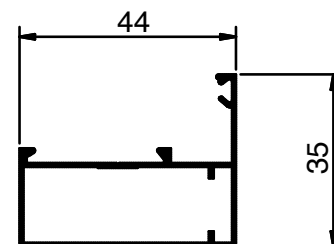
NC 1453 Weight: 0.340 KG/M
