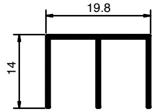
ST 7004 Weight: 0.125 KG/M
