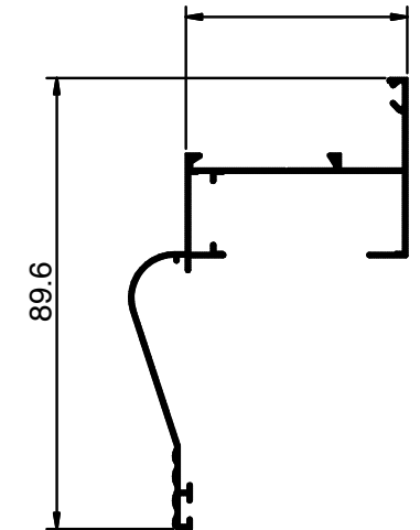
NC 1479 B Weight: 0.475 KG/M
