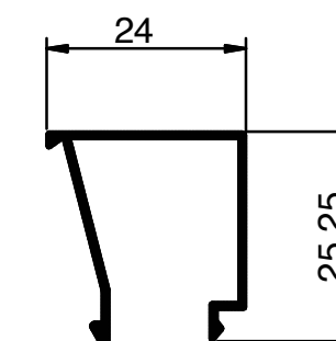
MR 707 Weight: 0.207 KG/M
