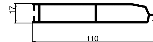
1201 Weight: 0.875 KG/M
