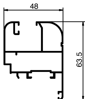
PS 4810A Weight: 0.710 KG/M
