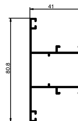
MR 702 Weight: 0.722 KG/M
