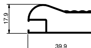
▶ IF 550 Weight: 0.248 KG/M
