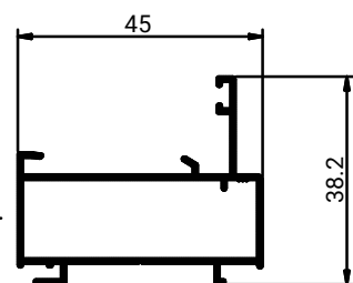
3937 Weight: 0.440 KG/M
