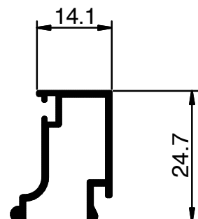
502 Weight: 0.229 KG/M
