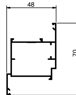
NC 1413 Weight: 0.508 KG/M
