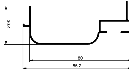
SOLAR 01 Weight: 0.408 KG/M
