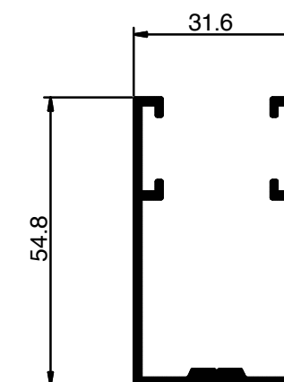
1200 Weight: 0.702 KG/M
