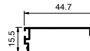
NC 1258 Weight: 0.170 KG/M
