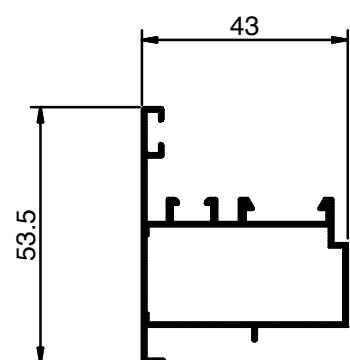
PS 4809 Weight: 0.480 KG/M
