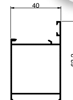
MR 140 Weight: 0.450 KG/M
