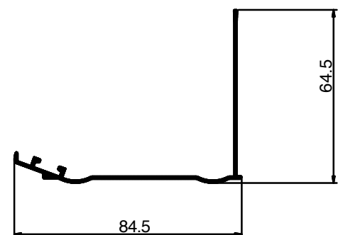
MR 807 Weight: 0.475 KG/M
