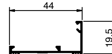
NC 1484 Weight: 0.180 KG/M
