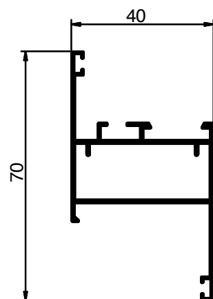
548 Weight: 0.625 KG/M
