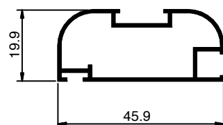
▶ IF 552 Weight: 0.278 KG/M
