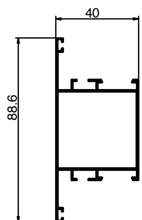
517 Weight: 0.780 KG/M
