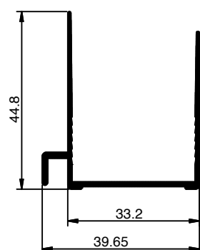
KW 08 Weight: 0.389 KG/M JOINT - PROFILE
