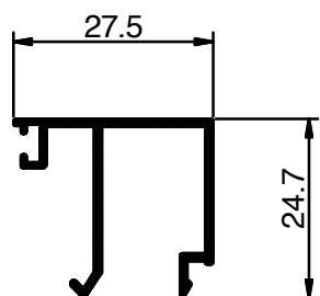
501 Weight: 0.265 KG/M
