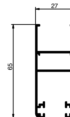
1.157 Weight: 0.665 KG/M
