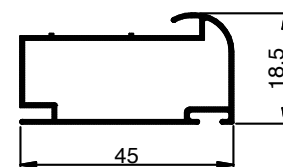
▶ IF 562 Weight: 0.286 KG/M
