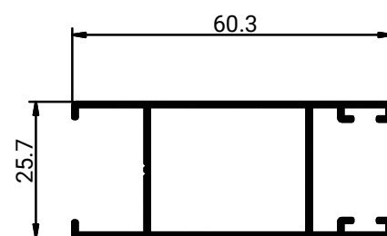
MR 1300 Weight: 0.515 KG/M
