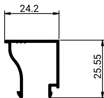
S 4008 Weight: 0.235 KG/M
