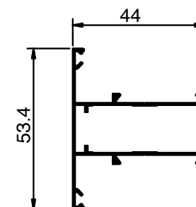
NC 1372 Weight: 0.425 KG/M
