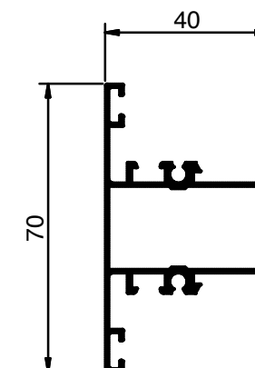
PS 4815 Weight: 0.666 KG/M
