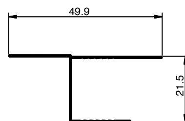
KW 07 Weight: 0.172 KG/M CHAIR - PROFILE
