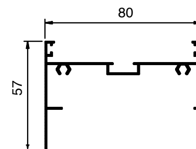
NC 1339 Weight: 0.534 KG/M
