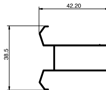
▶ IF 581 Weight: 0.275 KG/M
