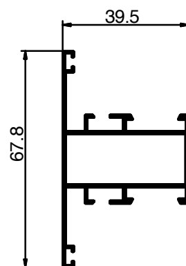
516 Weight: 0.680 KG/M
