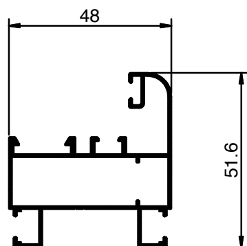
PS 4805 Weight: 0.490
