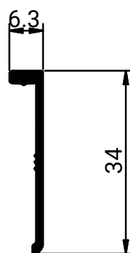
S 5002 Weight: 0.159 KG/M
