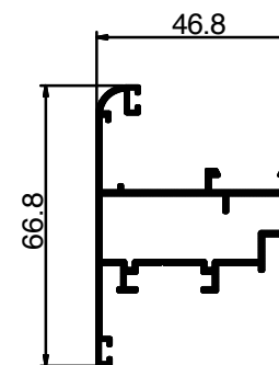
1.014 Weight: 0.721 KG/M
