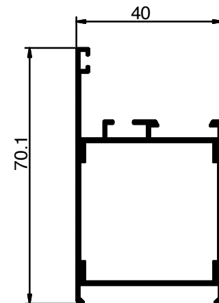
903 Weight: 0.735 KG/M
