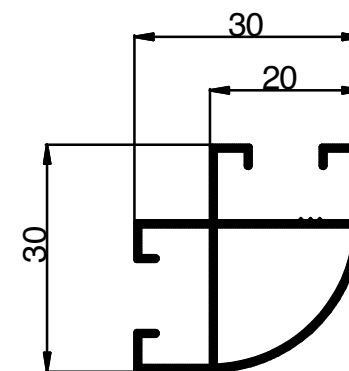
MR 304 Weight: 0.317 KG/M
