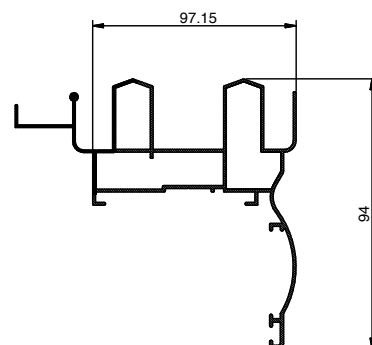
PS 6621 Weight: 1.012 KG/M
